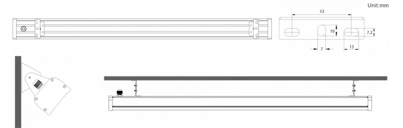
Wall Mounting
