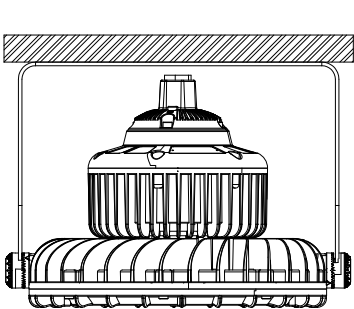
Ceiling Mounted
