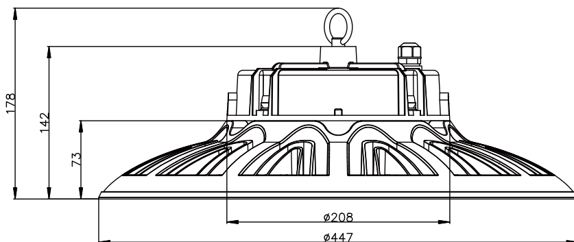
06 LGS-UFOB-400W/500W
