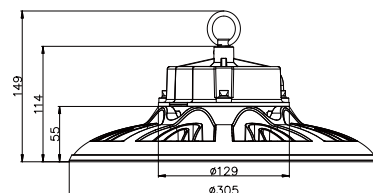
04 LGS-UFOB-200W/240W
