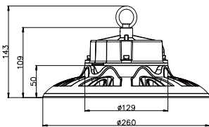
02 LGS-UFOB-100W
