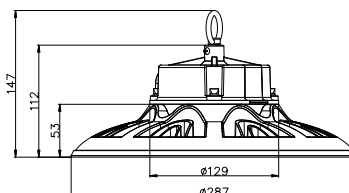
06 LGS-UFOB-400W/500W
